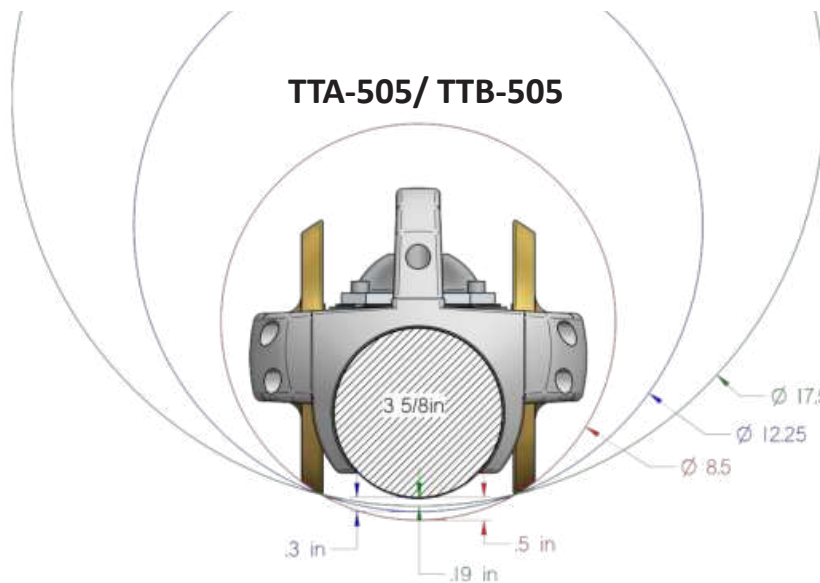
Figure 1: Standoff on a 3-5/8" Tool
