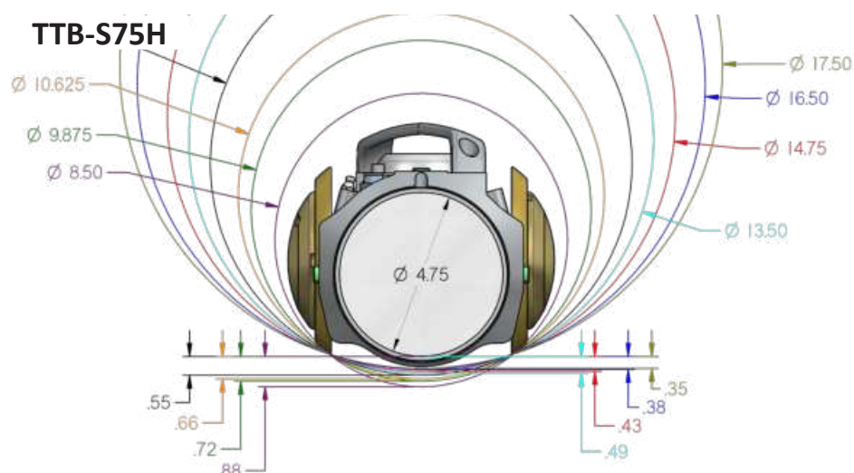
Figure 6: TTB - S75H Standoff for a 4- 3 / 4 " Tool
